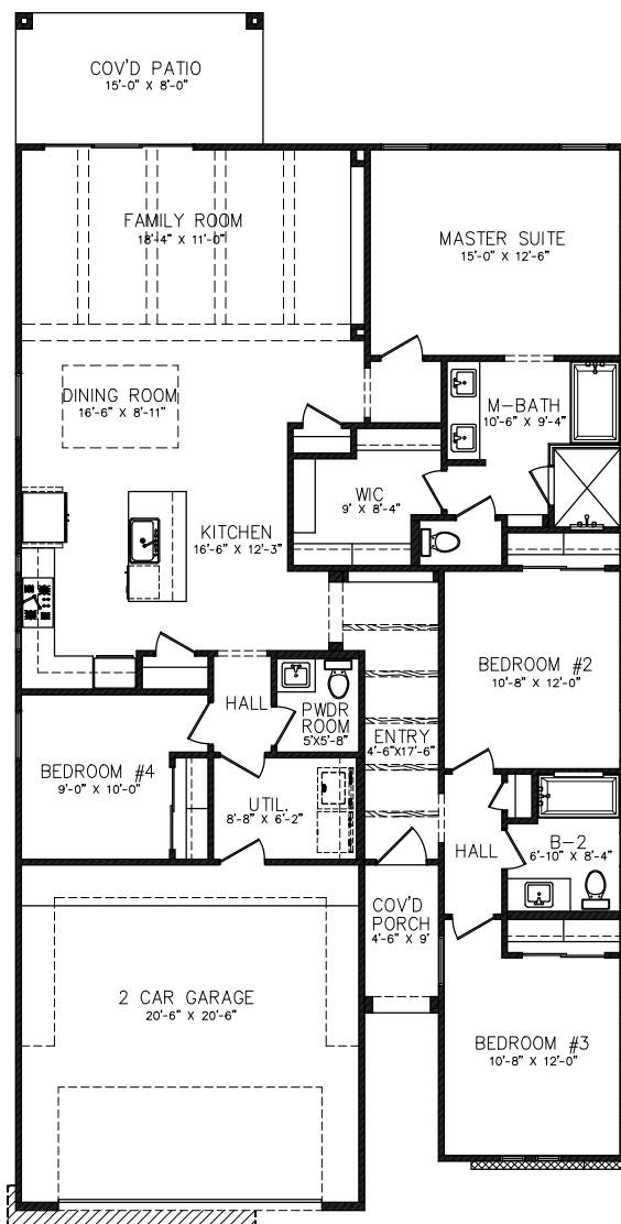
FLOOR PLAN
