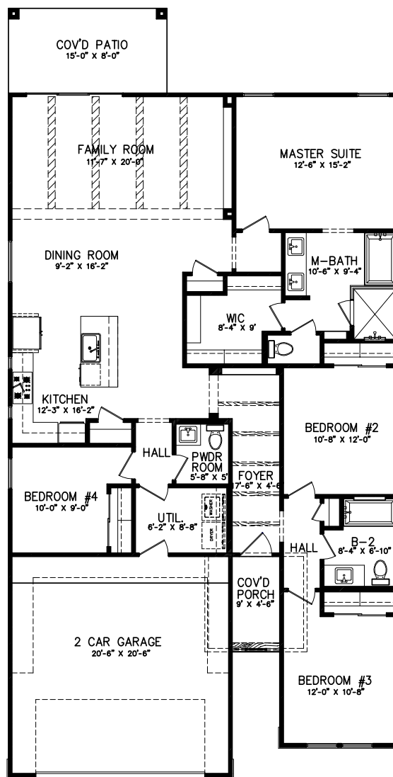
FLOOR PLAN
