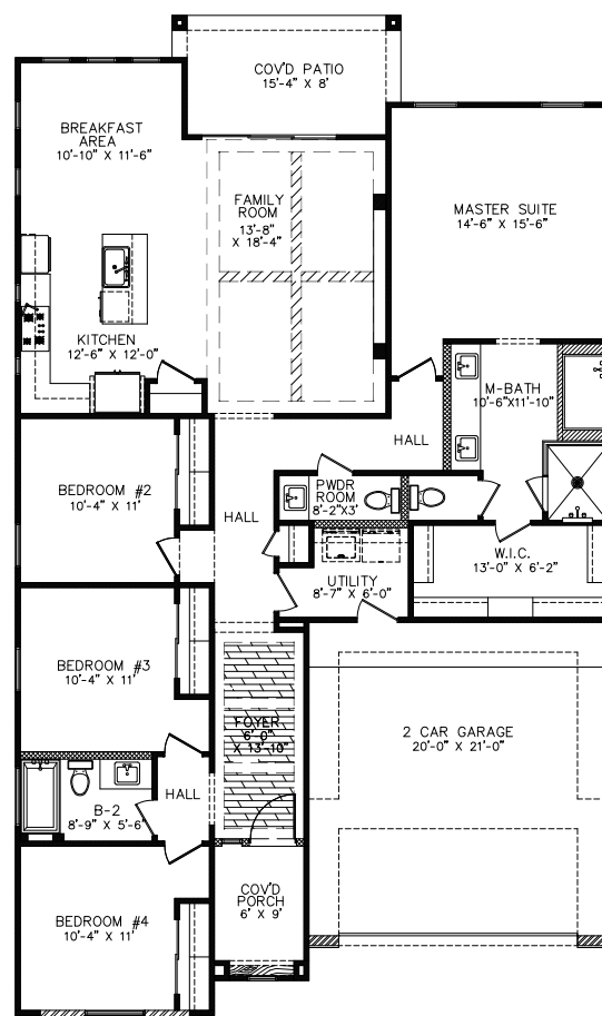
FLOOR PLAN
