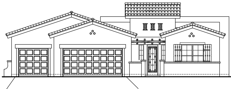
FRONT ELEVATION W/ CRTYRD
