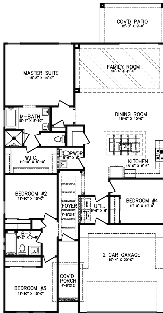
FLOOR PLAN
