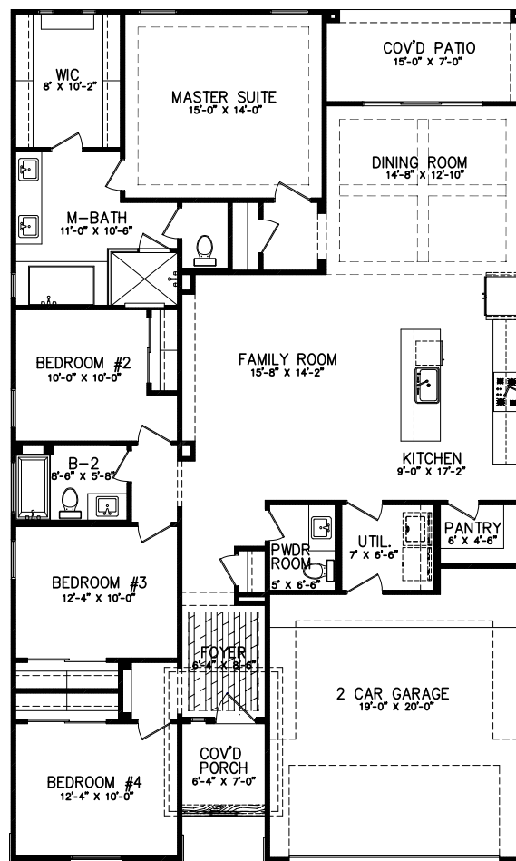
FLOOR PLAN
