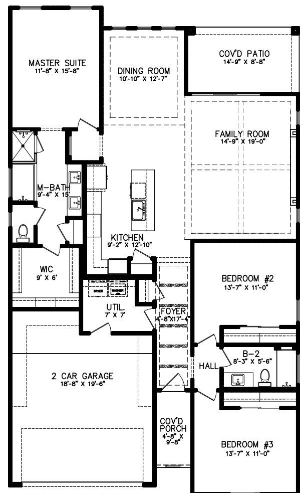
FLOOR PLAN
